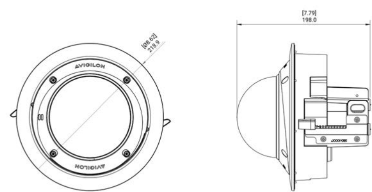
H6A Dome Camera with In-Ceiling Mount (CLADP-1001)
